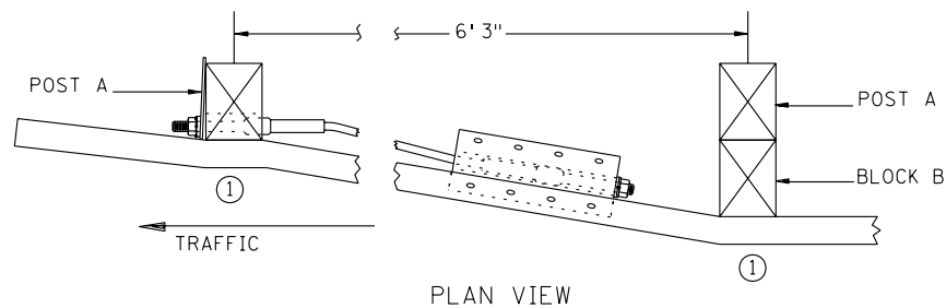
STRUT ANCHORAGE ASSEMBLY
